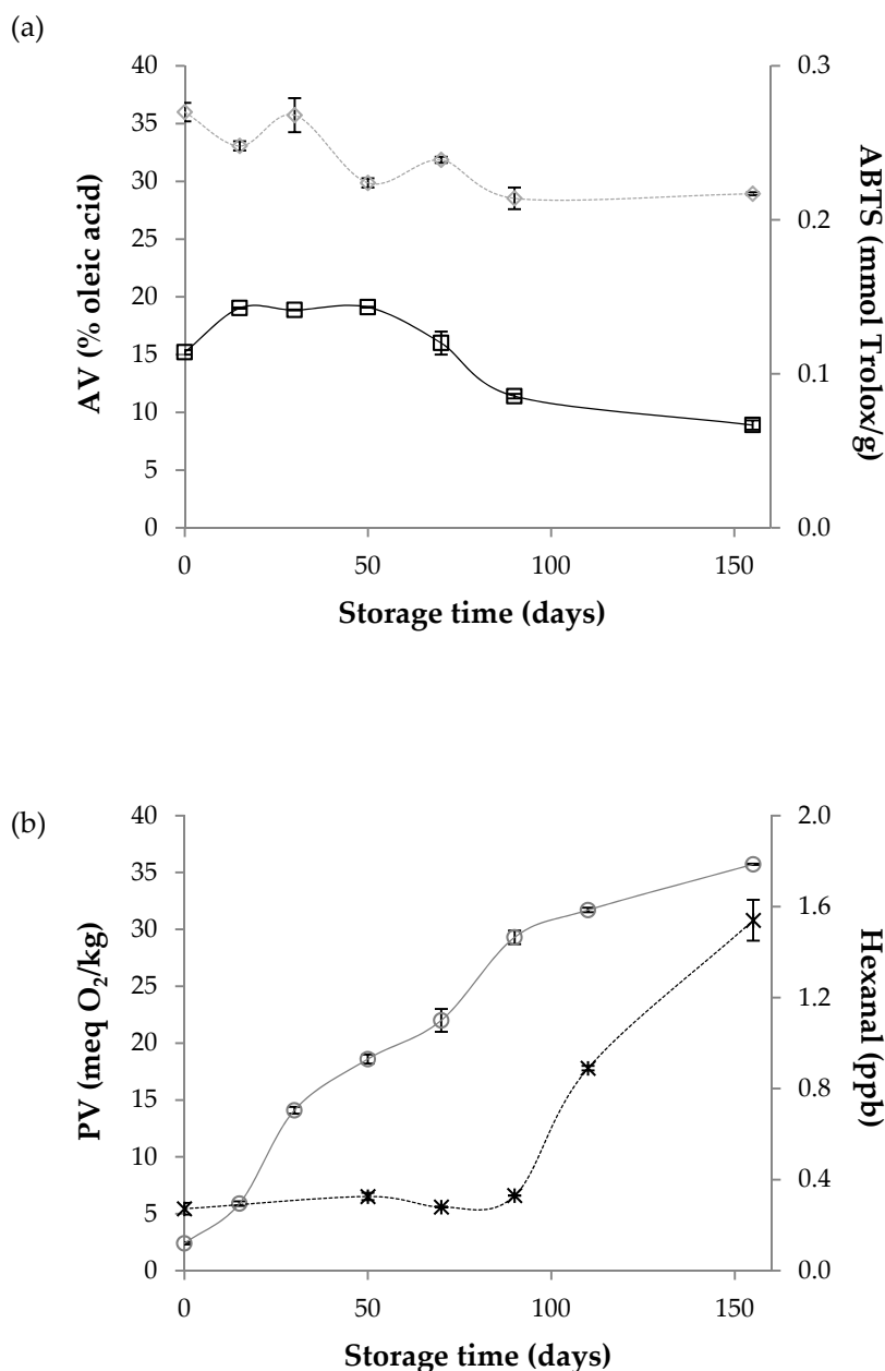
Figure 3. Evolution of: (a) □ acidity value (AV) and ◇ antioxidant activity (ABTS values) and (b) ○ peroxide value (PV) and × hexanal content, of the SCWBOE, measured during a storage period of 155 days at 21 ± 1 °C and in darkness.
