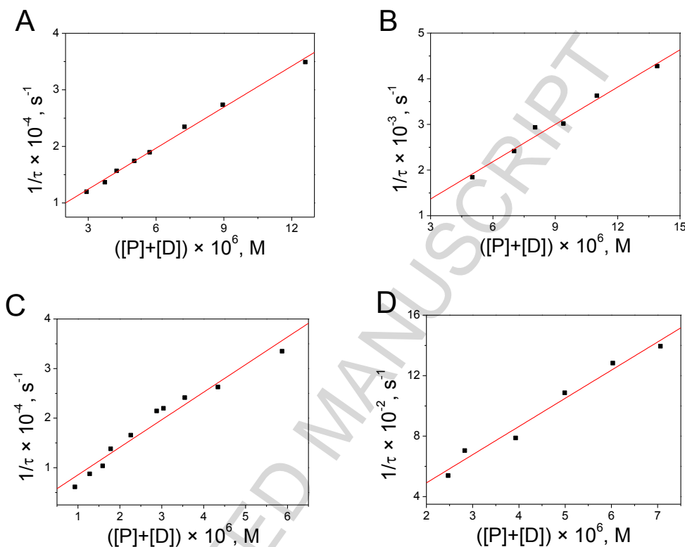
Fig. 5. (1/\tau) versus ([P] + [D]) plot and fitting of eqn (3) to the data obtained for the Tel22/TMPyP4 system in 0.15 M NaCl at (A) \lambda = 437 \text{ nm} , and (B) \lambda = 422 \text{ nm} and in 0.15 M KCl at (C) \lambda = 437 \text{ nm} and (D) \lambda = 422 \text{ nm} .
