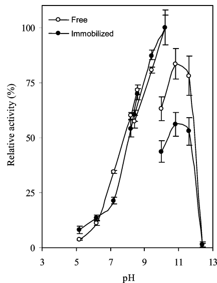
Figure 3. pH/activity curves for free and immobilized alkaline phosphatase. Reaction conditions: 0.1 M Tris-maleate (pH 5.2–8.6), 0.1 M borate (pH 8.4–10.2), and 0.1 M glycine (pH 10–12.4); incubation temperature, 37 °C; reaction time, 60 min; 25 mM pNPP. Relative activity was expressed as a percentage of maximum activity under experimental conditions.
