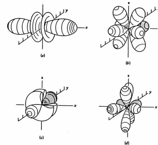
Figure 2-18 Representations of 4f orbitals. (a) f_{x(5x^2-3r^2)} ; (b) f_{x(z^2-y^2)} ; (c) f_{y(5y^2-3r^2)} ; (d) f_{y(z^2-x^2)} [J. T. Waber and J. E. Hockett, in Proceedings of the Fourth Conference on Rare Earth Research , L. Eyring (Ed.), Fig. 3, p. 287, Gordon and Breach, New York (1965).]
