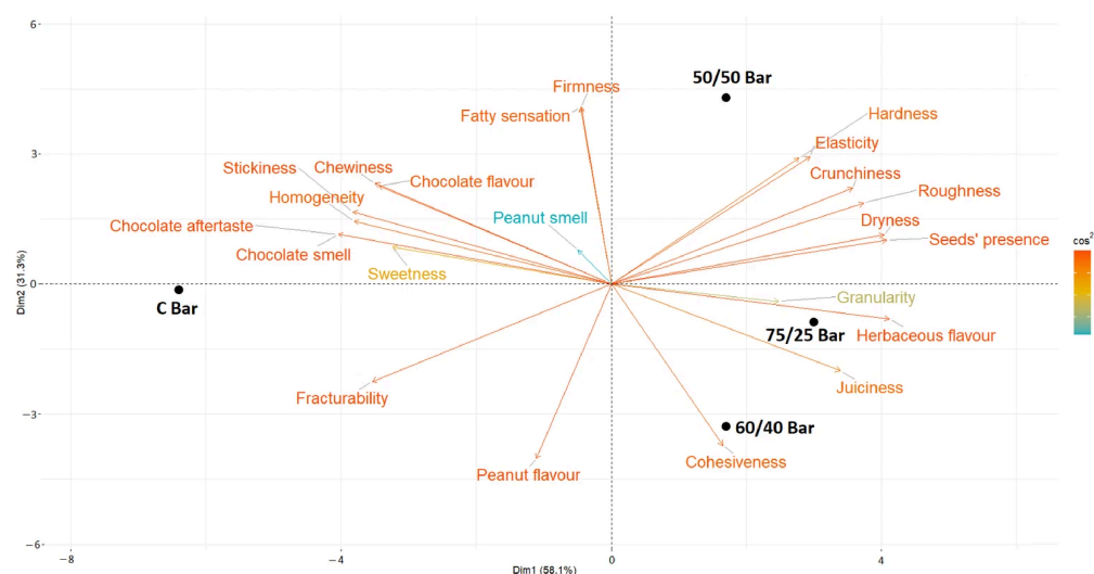
Figure 3. Biplot map of Generalised Procrustes Analysis performance based on Flash profile results. Variable importance on each axis is represented by \cos^2 (an indicator of variable quality representation; the closer to 1, the more the variable contributes to the corresponding axis).
