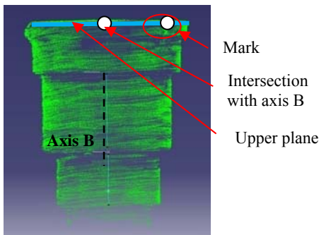
Fig. 7. Rivet Pin references.
