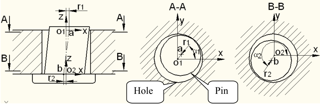
a) Cross-sectional side view b) Cross-sectional top view at a and b
