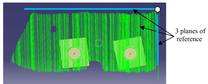
Fig. 8. . Base plate references.
