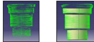
Fig 6. Generating features
