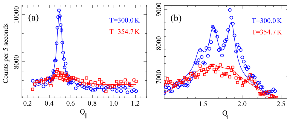
Figure 3. Examples of the neutron scattering intensity as a function of Q_{\parallel} for (a) the low- Q and (b) high- Q Bragg peaks. The Q units are in \text{\AA}^{-1} . The scans were made at constant Q_{\perp} = 0.23 \text{\AA}^{-1} and Q_{\perp} = 0.6 \text{\AA}^{-1} for the low- and high- Q peaks respectively. Examples of fits, as explained in the text, are also shown.
