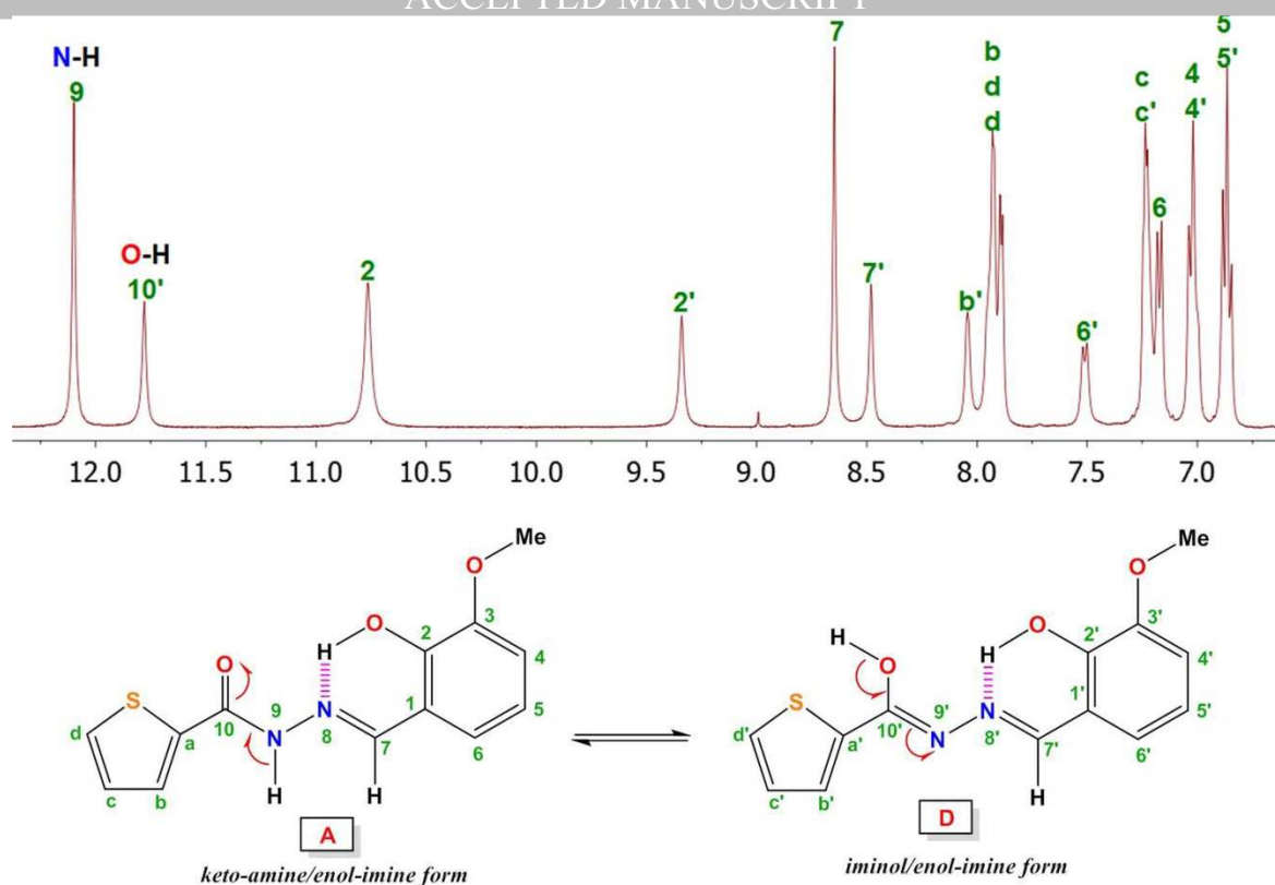
Figure 5. Possible tautomeric equilibria for oVATPNNH. Low field region of the ^1\text{H} NMR spectrum recorded in \text{CD}_3\text{SOCD}_3 at 25^\circ\text{C} , showing two sets of resonances with an integral ratio (2:1) in agreement with a slow dynamic equilibrium between two tautomers. The OMe signals of both tautomers are accidentally isochronous.
