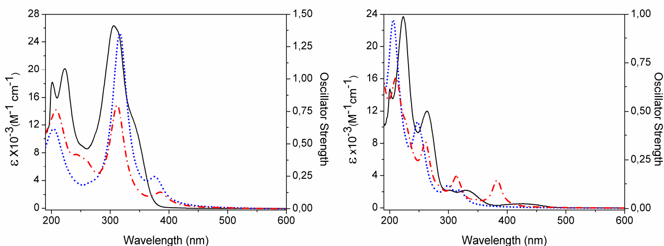
Figure 7. Electronic spectra of o VATPNNH (left panel) and o VATPNH2 (molecule 1 , right panel) in EtOH. Experimental (—), and calculated for tautomers A (.....) and D or B ( - ); respectively.
