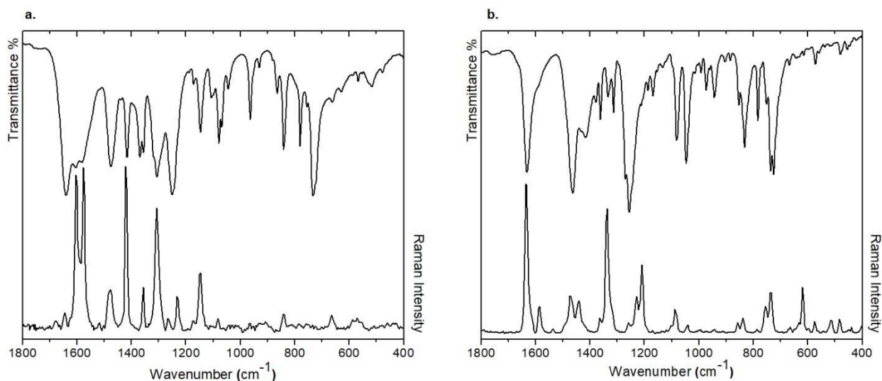
Figure 2. IR and Raman spectra of a) oVATPNNH.H 2 O (1) and b) oVATPNNH 2 (2) in the more relevant spectral region.
