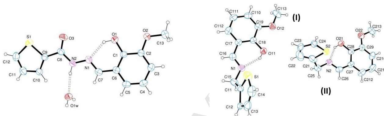
Figure 1. View of oVATPHNNH.H 2 O ( left ). Part of the H-bonding pattern is drawn by dashed lines. Plot of the asymmetric unit content of oVATPNH2 ( right ) showing the labeling of the non-H atoms and their displacement ellipsoids at the 30% probability level for each independent molecule ( I and II ). The graph depicts only one of the two conformations exhibited by the rotationally disordered thiophene ring of molecule ( II ). Intra-molecular H-bonds are indicated by dashed lines.
