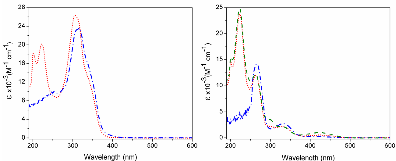
Figure 6 Electronic spectra of both compounds in the 190-600 nm range. Left: oVATPNNH in solution of DMSO (- . - . -), EtOH (.....); Right: oVATPNH 2 in DMSO (- . - . -), EtOH (.....) and MeOH (- - -)
