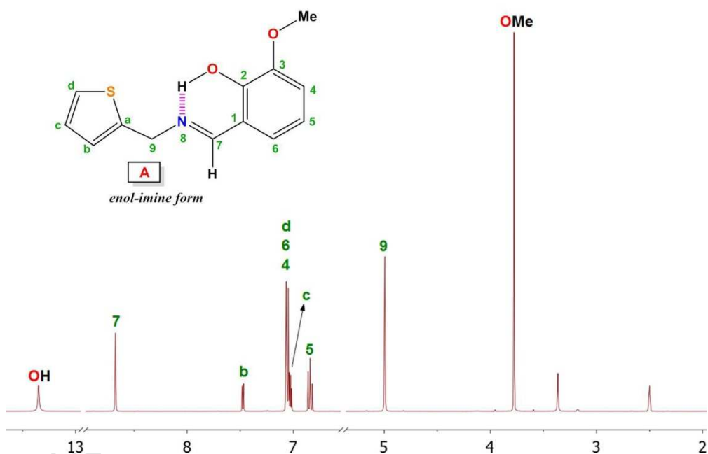
Figure 4. ^1\text{H} NMR spectrum recorded for o VATPNH2 in \text{CD}_3\text{SOCD}_3 at 25 ^\circ\text{C} , showing only one set of resonances in agreement with the presence of one tautomer (A). Two cuts have been applied for the sake of clarity.
