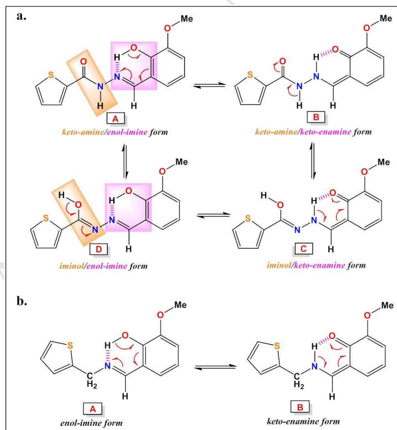
Figure 3. General outline showing all the possible tautomers for: a) oVATPNNH and b) oVATPNNH 2 .
