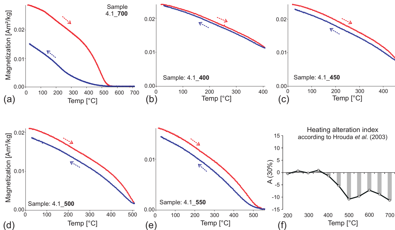
Figure 7 (a) High-temperature thermomagnetic curve (magnetisation vs. temperature) up to 700 °C of the limestone sample 4.1 after the experimental heating. (b-e) Partial thermomagnetic curves in 50 °C incremental steps from 200 °C to 700 °C carried out on an additional fragment of the sample 4.1. For clarity, panels b-e only show steps from 400 °C to 550 °C. Heating (cooling) cycles are plotted in red (blue) with their respective arrows. Sample code and magnetisation intensity values are also shown. (f) Histogram showing the variation in the alteration index of individual heating/cooling runs of 4.1 limestone sample following Hrouda's et al. (2003) method. See section 3.2 for explanation.
