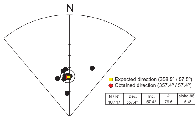
Figure 8 Stereoplote showing the mean archaeomagnetic direction obtained (red circle) and the expected direction (yellow square). Archaeomagnetic directional results are shown with their corresponding Fisher (1953) statistical parameters. N = samples considered for calculation; N' = total number of samples processed; Dec = declination; Inc = inclination, k and \alpha_{95} = precision parameter and 95% confidence limit of characteristic remanent magnetisation, respectively.
