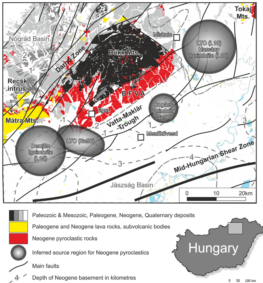
Fig. 12. Inferred volcanic source regions for various pyroclastic deposits of the BFVA (Sz98 – Szakács et al., 1998; L10 – Lukács et al., 2010; L15 – Lukács et al., 2015) in relation with structural units and zones of Neogene-Quaternary subsidence. LTC is Lower Tuff Complex including the Eger and Mangó Ignimbrites. Basemap: surficial geological map of Hungary published by the Mining and Geological Survey of Hungary ( https://map.mbfisz.gov.hu/fdt100/ ). Fault lines were adopted from Beke et al. (2019) and the Neogene basement isolines from Horváth and Royden (1981).
