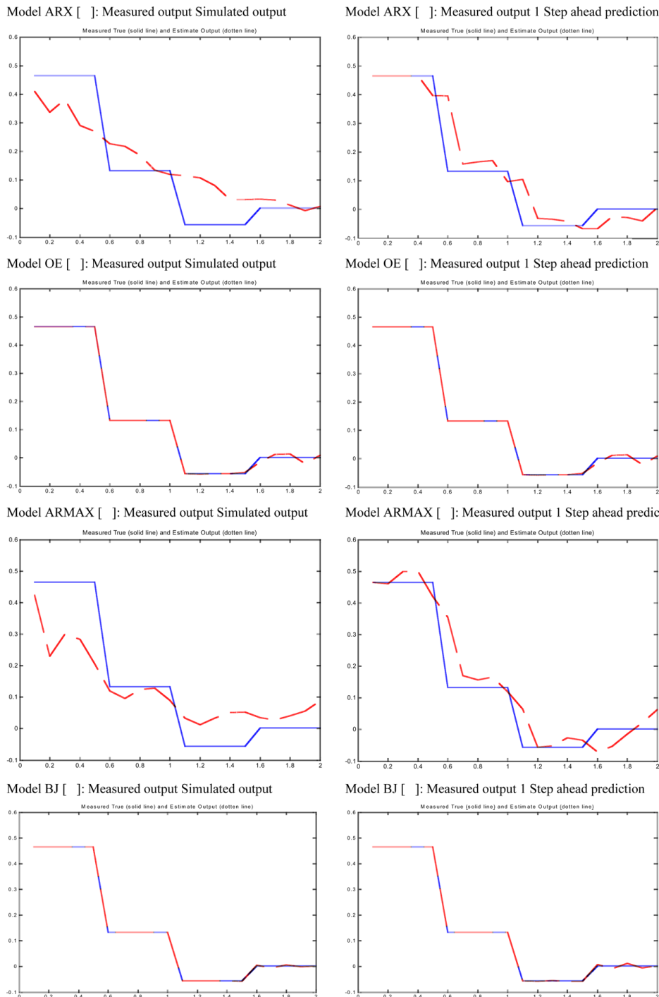
341 Figure 2. Representation of system output, simulated output and one-step-ahead prediction for four black-box models. 342 The order of the structure of the model is n_a = 4, n_b = 2, n_c = 3, n_d = 2, n_f = 4, n_k = 3 [4, 2, 3, 2, 4, 3] according to 343 the model type. The solid line represents the output variable and the dashed line represents estimated output. 344 345 346 347 348 349 350
