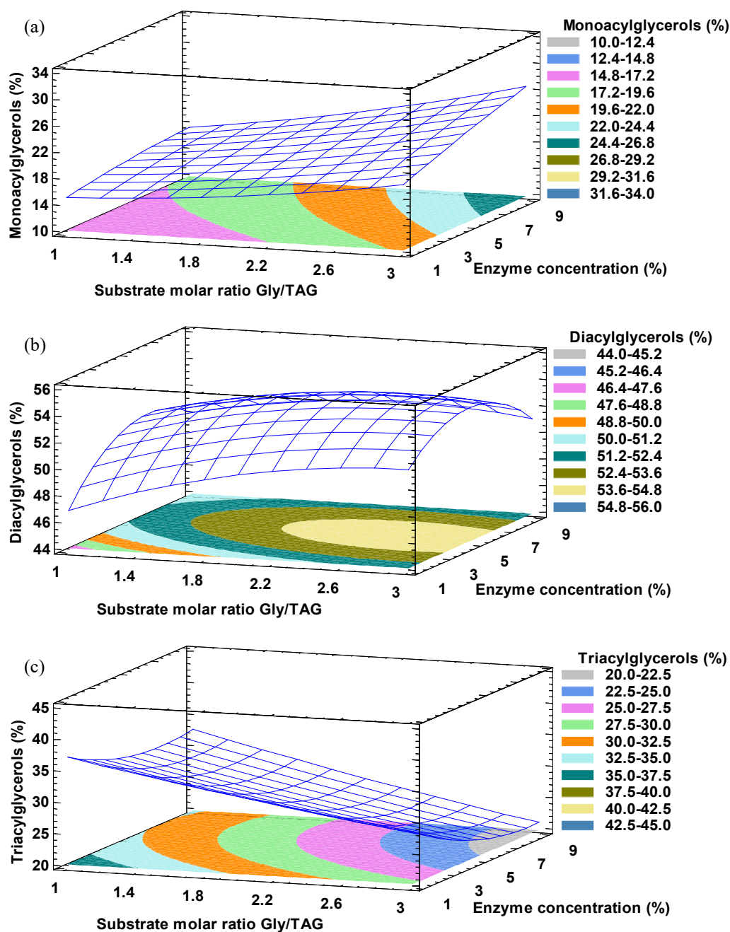
Fig. 1. Response surface plots showing the effect of substrate molar ratio and enzyme concentration on (a) MAG production, (b) DAG production, and (c) TAG consumption, during solvent-free glycerolysis with Lipase PS-DI. The reaction took place at 50 °C for 4 h at 200 rpm.
