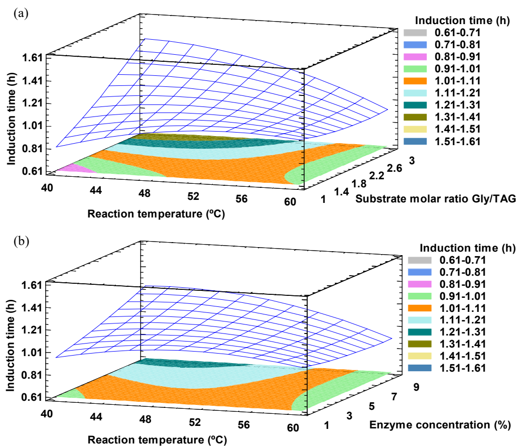
Fig. 3. Response surface plot of the oxidative stability of the solvent-free glycerolysis products. (a) Effect of reaction temperature and substrate molar ratio (Gly/TAG) on induction time, with 5% of Lipase PS-DI; (b) Effect of reaction temperature and enzyme concentration on induction time, with Gly/TAG molar ratio of 2/1.
