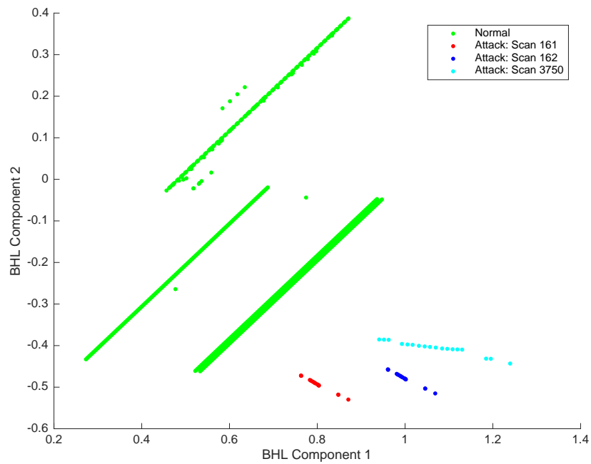
Figure 2. BHL projection for dataset 1, port scan attack.
