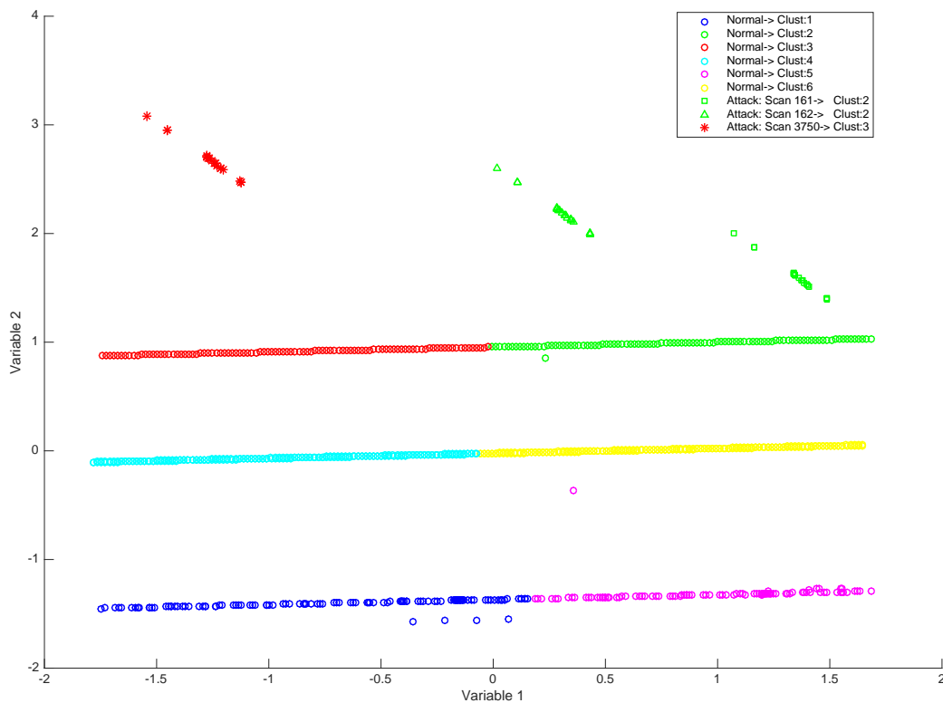
Figure 3. MOVICAB projection for dataset 1, port scan attack.
