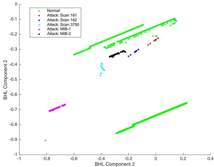
Figure 6. BHL projection for dataset 3, MIB transfer and port scan attacks.
