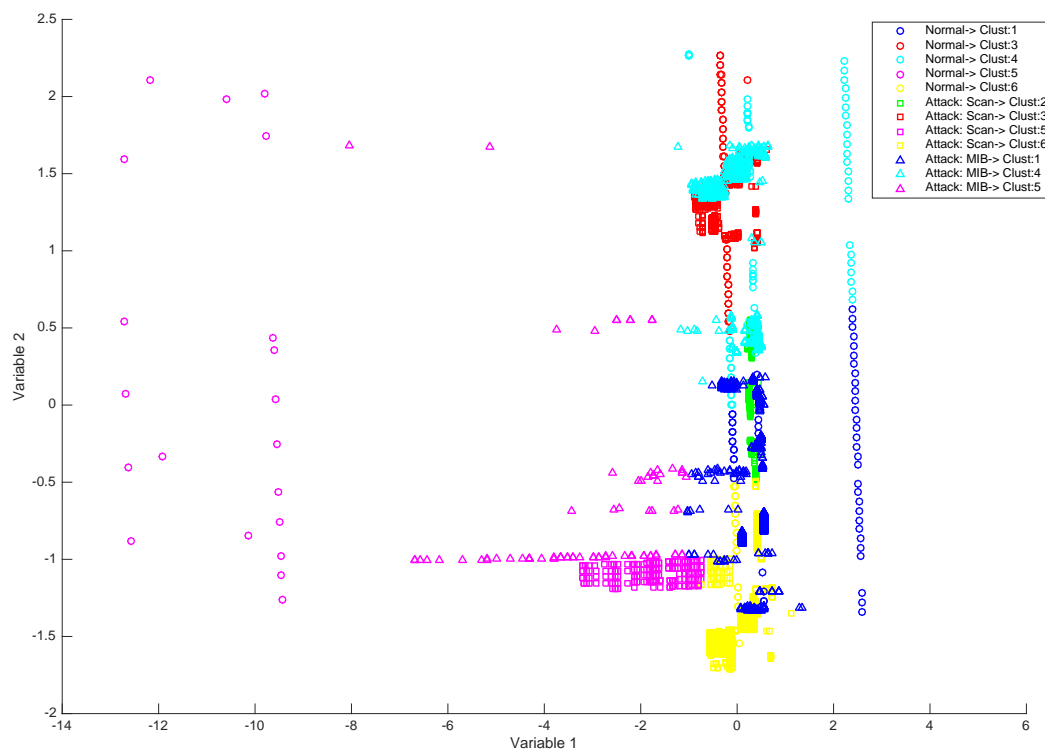
Figure 7. MOVICAB projection for dataset 3, MIB transfer and port scan attacks.
