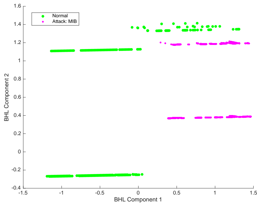
Figure 4. BHL projection for dataset 2, MIB transfer attack.
