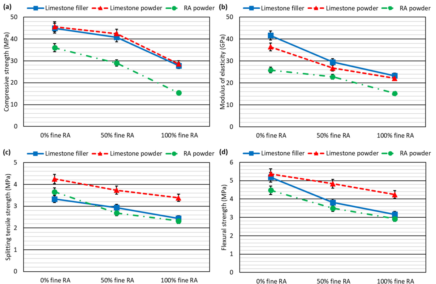
Figure 3. Mechanical performance of SCC mixes: (a) compressive strength; (b) modulus of elasticity; (c) splitting tensile strength; (d) flexural strength.
