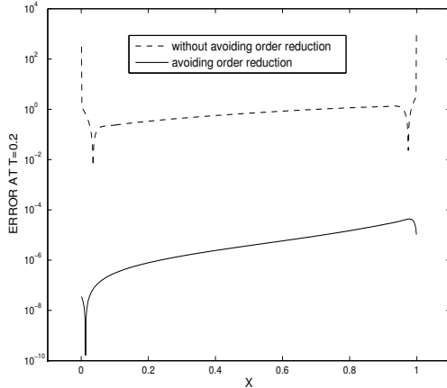
Figure 2: Error at each node at final time when integrating the one-dimensional problem corresponding to data (54) and (55) avoiding and not avoiding order reduction with Strang
