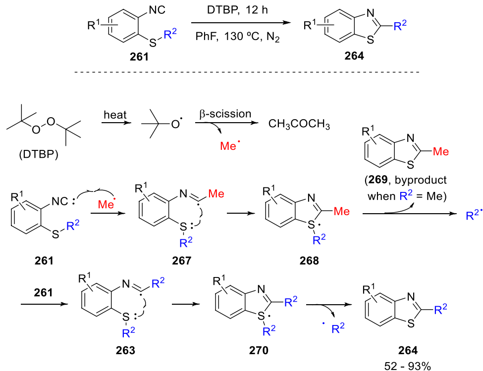
Scheme 48 Radical synthesis of benzothiazoles by reinstallation of the alkyl substituent
