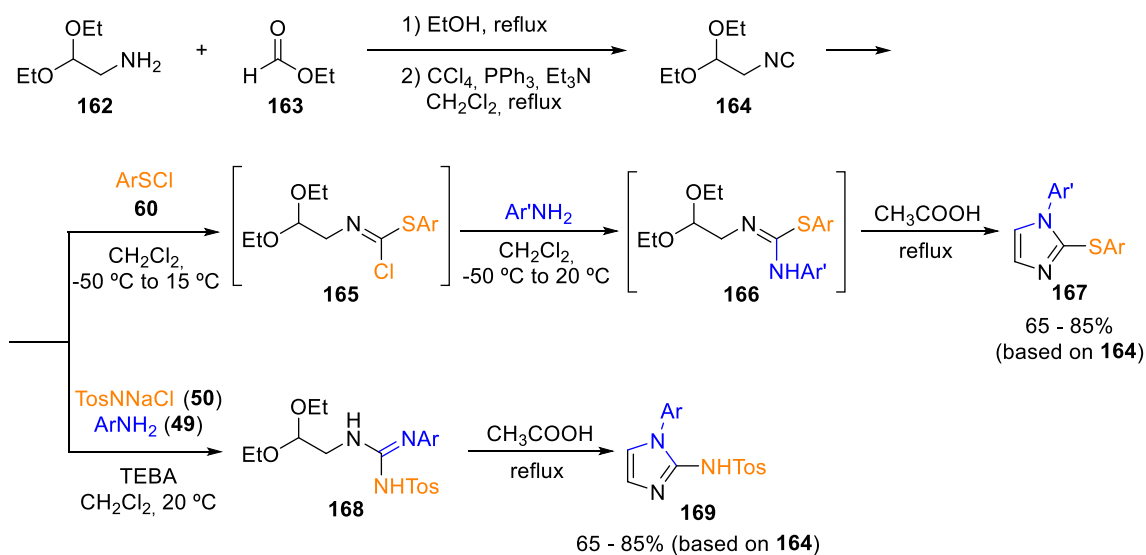
Scheme 27 2,2-Diethoxyisocyanohydrin in heterocyclic synthesis
