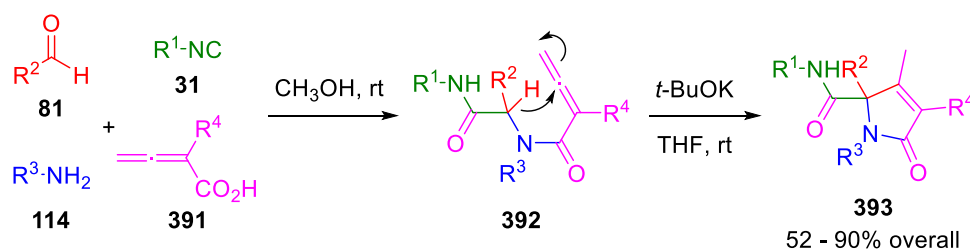
Scheme 78 Balaia's synthesis of pyrrolidinones
