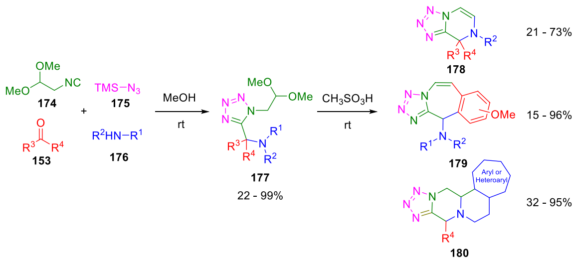
Scheme 29 Synthesis of diverse heterocyclic scaffolds employed 2,2-diethoxyisocyanohydrin
