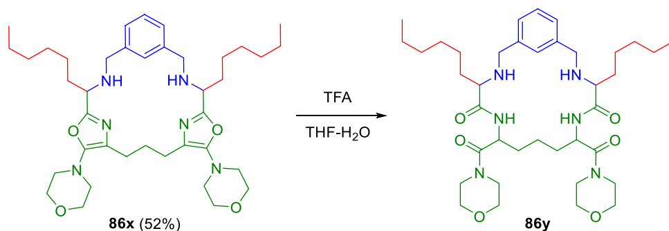
Scheme 15 Zhu's oxazole synthesis from isocyanoacetamides
