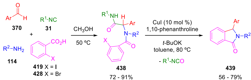
Scheme 88 Deamidative \text{C}(\text{sp}^2)\text{-C}(\text{sp}^3) coupling for the synthesis of isoindolinones
