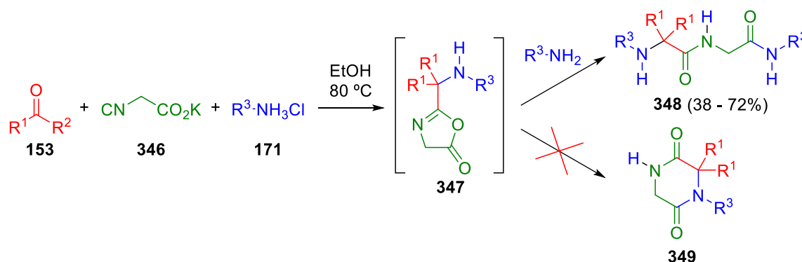
Scheme 67 Synthesis of dipeptides from potassium isocynoacetates
