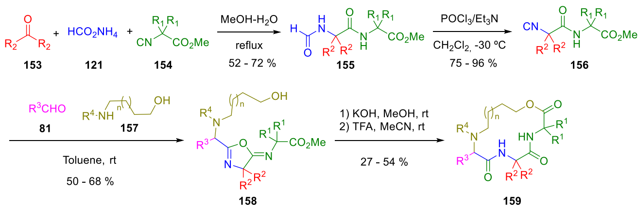
Scheme 25 Macrocyclodepsipeptides construction employing isocyanoacetamides
