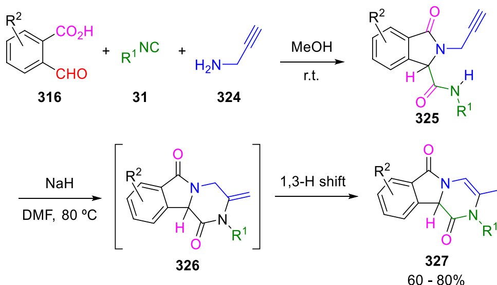
Scheme 62 Synthesis of pyrazino[2,1- a ]isindolediones
