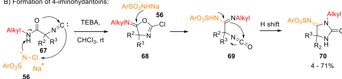
Scheme 12 Regioselective synthesis of iminohydantoins
