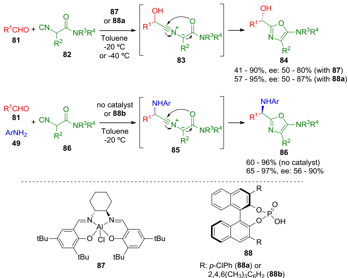
Scheme 15 Zhu's oxazole synthesis from isocyanoacetamides
