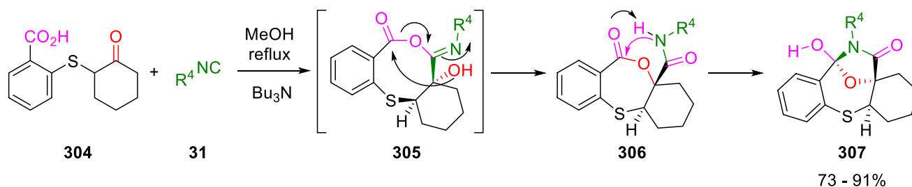
Scheme 56 Intramolecular Passerini condensation to prepare tetracyclic 1,4-benzothioxepin orthoamides
