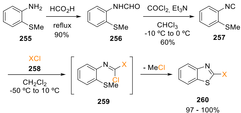
Scheme 45 2-Functionalised benzothiazoles from 2-isocyanatoanisole
