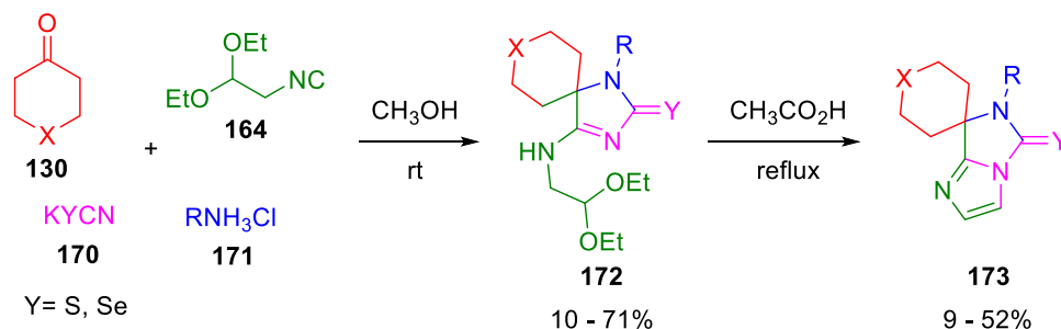
Scheme 27 2,2-Diethoxyisocyanohydrin in heterocyclic synthesis
