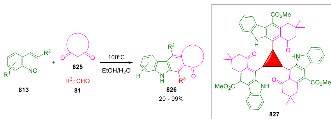
Scheme 176 Tandem Knoevenagel/[4+1]/intramolecular [4+2] cycloaddition to cyclo[ b ]fused carbazoles
